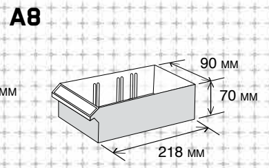
A8 A8 Cabinet Drawer
