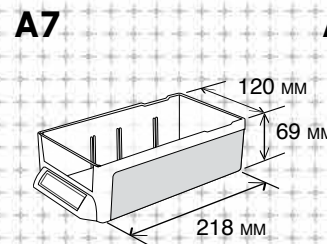
A7 A7 Cabinet Drawer
