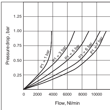
3/4" LUBRICATOR
