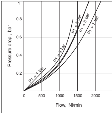
1/4" LUBRICATOR
