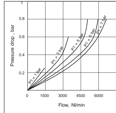
1/2" LUBRICATOR
